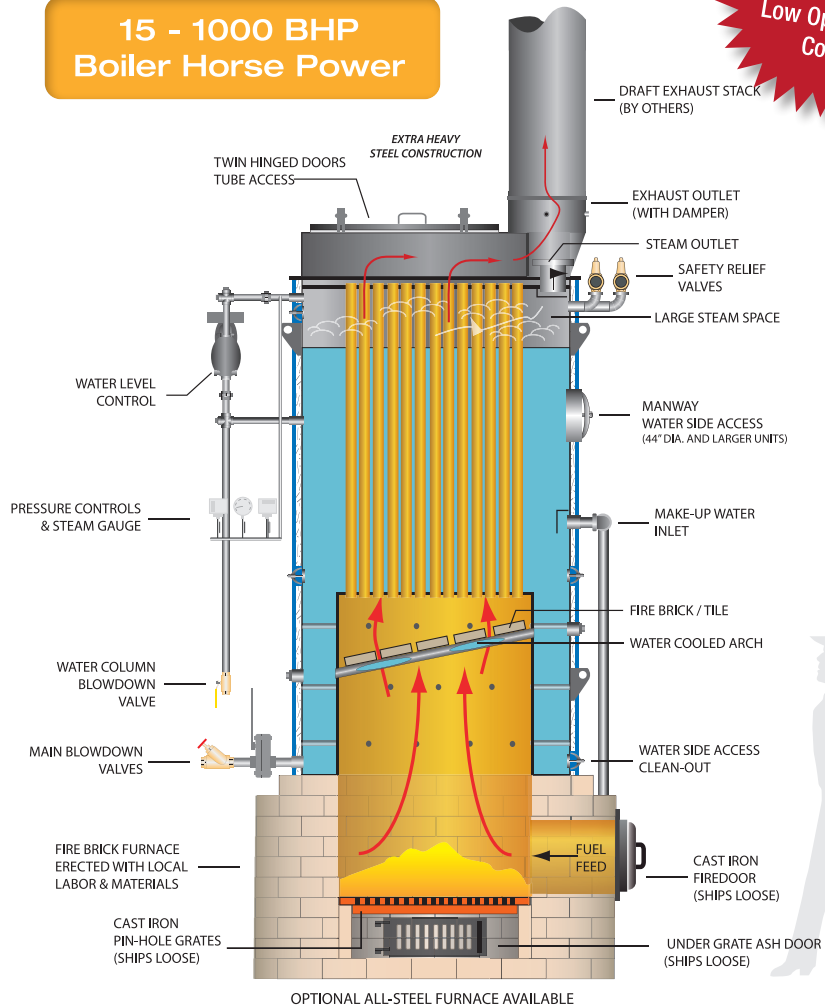
OPTIONAL ALL-STEEL FURNACE AVAILABLE
