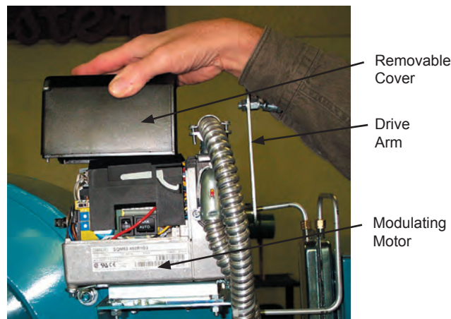
Figure B-25 Landis Mod Motor Adjustments
